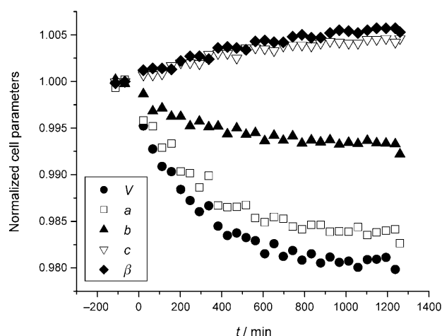
Figure 3. Unit-cell parameters as a function of time. The laser is turned on at t=0 min. The standard deviation values are smaller than the symbols used in the plot. Unit-cell parameters have been calculated for each of the 32 separate \omega scans.
